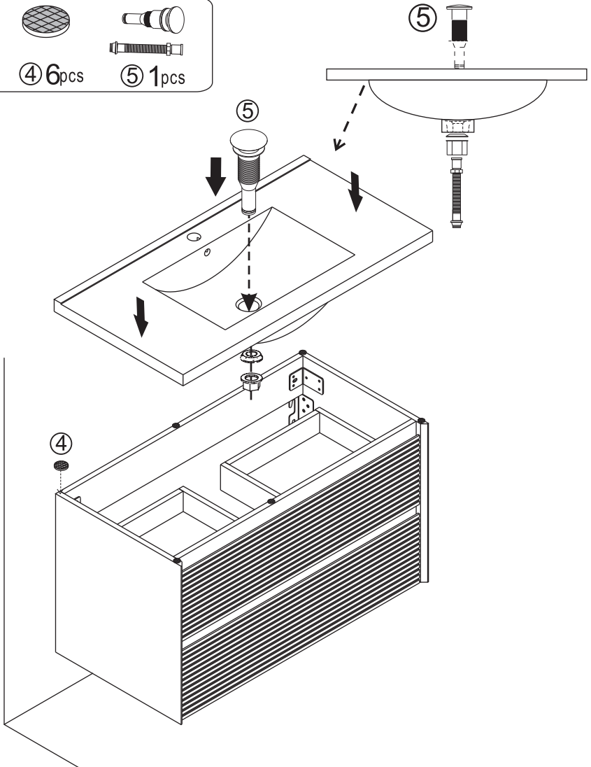
Installation of drain assembly
