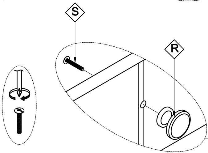
STEP 22
